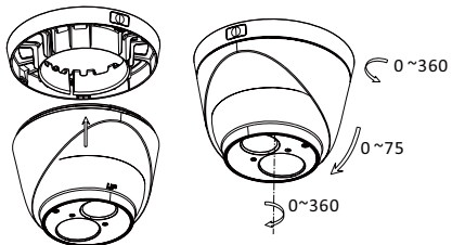
Figure 2-3 3-axis Adjustment
