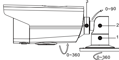
Figure 2-7 3-axis Adjustment
