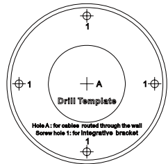
Figure 2-5 Drill Template
