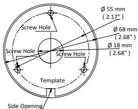
Figure 2-1 Drill Template
