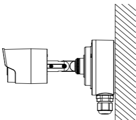
Figure 2-7 Fix the Junction Box Cover back to its Body
