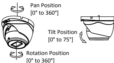
Figure 2-11 3-axis Adjustment
