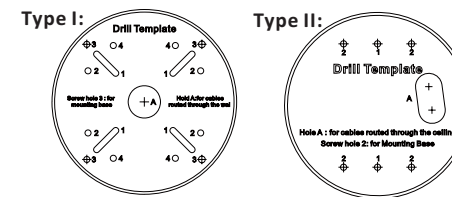
Figure 2-1 The Drill Template
