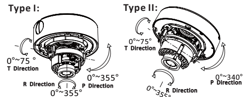
Figure 2-4 3-axis Adjustment
