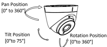
Figure 2-5 3-axis Adjustment
