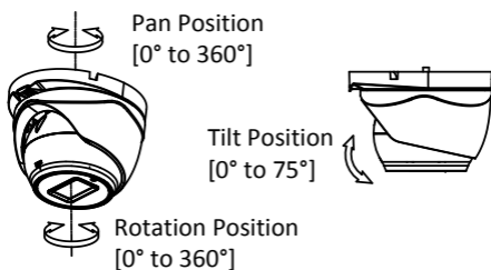
Figure 2-11 3-axis Adjustment
