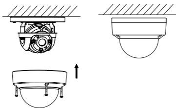
Figure 2-10 Bubble Reinstallation
