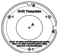
Figure 2-1 Drill Template
