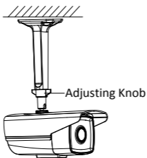
Figure 2-13 Install the Camera
