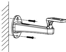
Figure 2-10 Fix the Bracket
