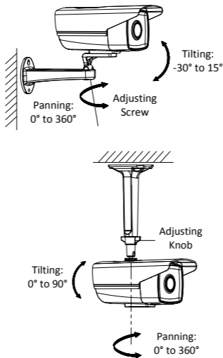
Figure 2-14 Adjust the Angle
