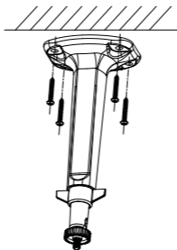
Figure 2-12 Fix the Bracket
