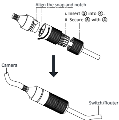
Figure 2-16 Waterproof Accessory Installation
