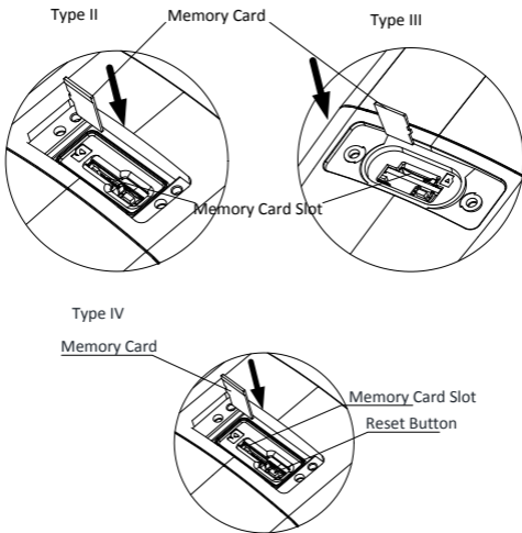
Figure 2-2 Insert Memory Card
