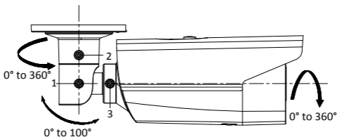
Figure 2-5 Adjust the Surveillance Angle
