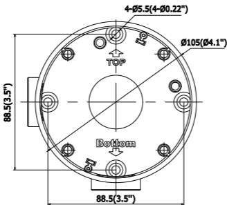
Figure 2-7 Dimension of Junction Box
